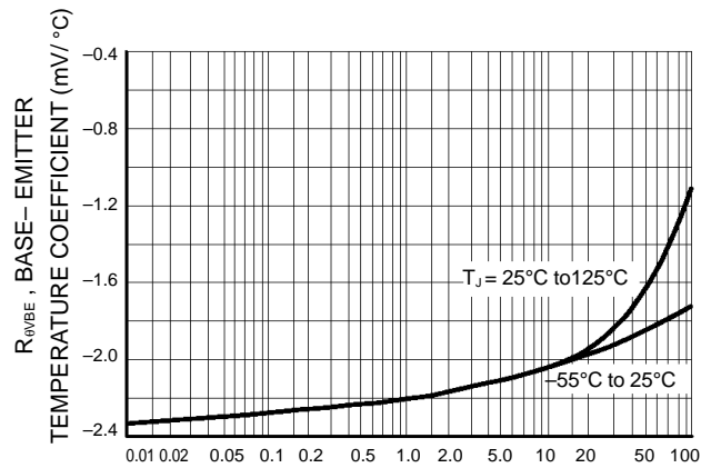
Figure 10. Temperature Coefficients
